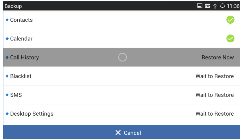
Figure 29: Restore Process
